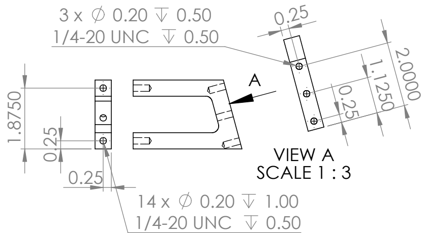
Corner Guard Bracket: 9/3/26
